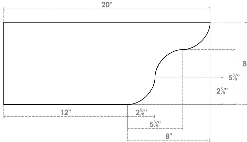
SIDE PROFILE
